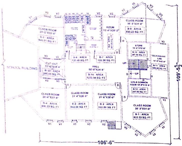
BASMENT FLOOR PLAN
